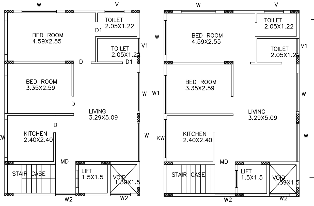
GROUND FLOOR PLAN TYPICAL FIRST AND SECOND FLOOR PLAN
